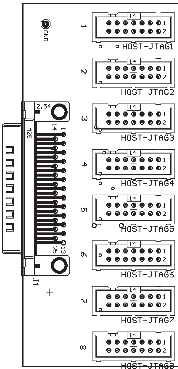
Figure 5-6. Gang_Exp Layout
